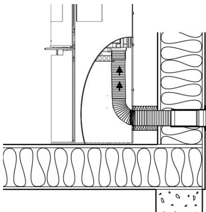
Through wall
