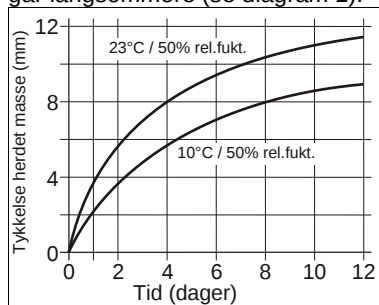
Diagram 1: Herdehastighet for Sikaflex®-291i
